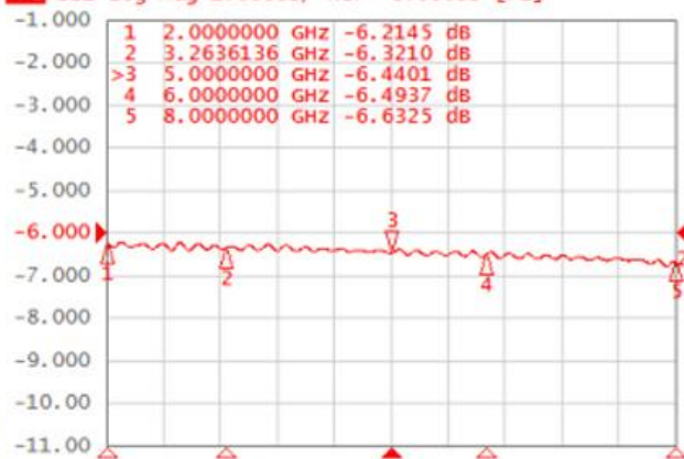
2.插入损耗 Insertion Loss
